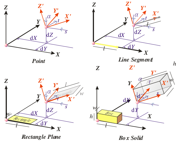
Figure 2: Pose parameters adjustment of floating models
