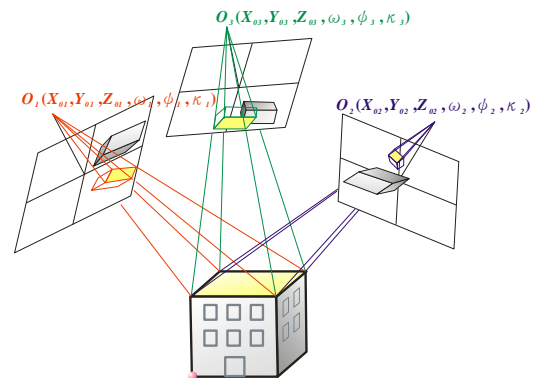
(a) Projection based on incorrect image orientation parameters
