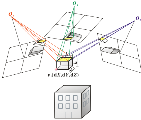
(b) Projection based on incorrect model parameters Figure 4: Precise image orientation and model parameters are both required for correct model projection
