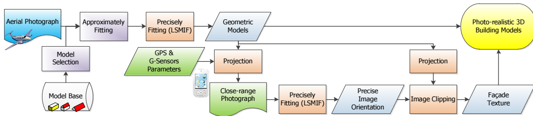
Figure 1: The proposed photo-realistic 3D building modelling procedure
